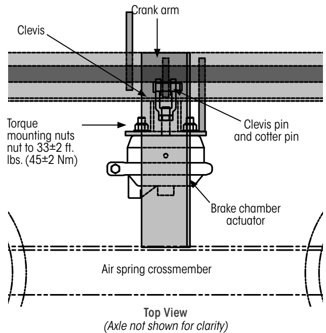
Figure 58: SLKU brake chamber actuator mounting bracket
