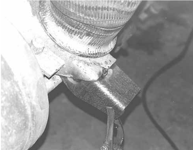
Figure 72: Tack weld rear beam extensions in place
