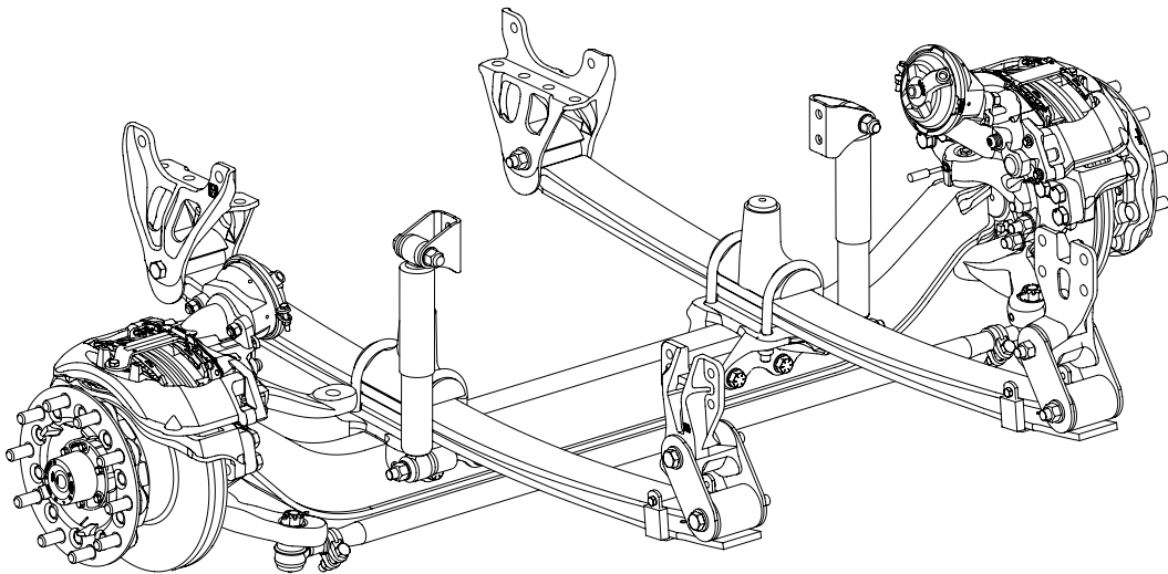
SOFTEK with STEERTEK NXT Axle 10K Shown
