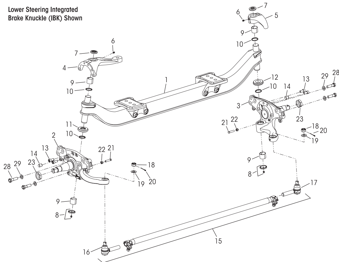
STEERTEK NXT Axle with Shock Absorber Lug, Vehicles built between August 2011 and January 2025
