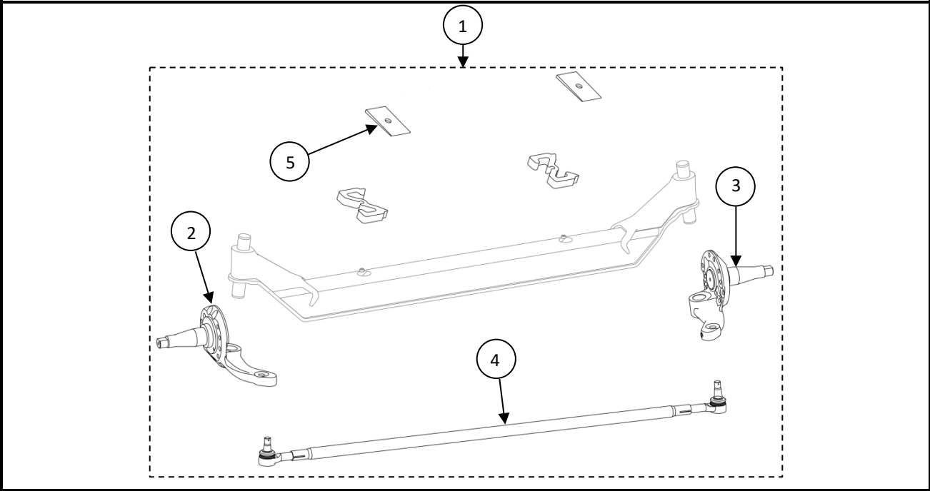
Front Suspension Assembly Part Number 97360-050
