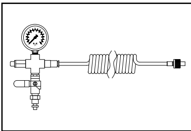
TIREMAAX PRO TARGET GAUGE Part No. VS-32331
