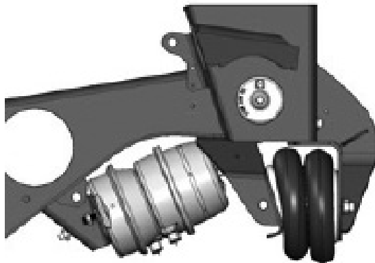
Figure 1: UBL-201 with TSE Ultralife 30/30 Long chamber
