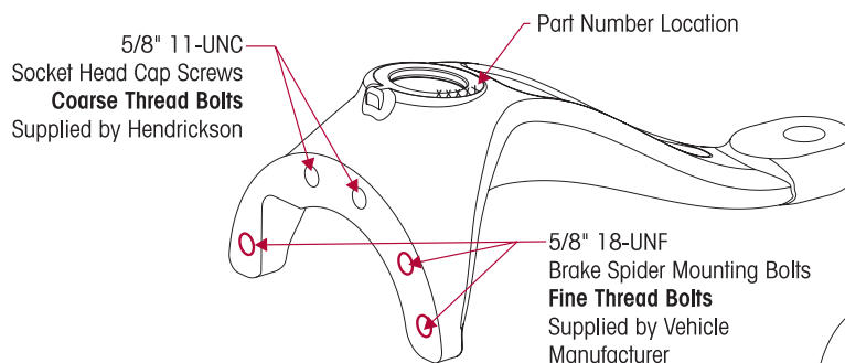
Figure 1 New Left Hand Upper Steering Knuckle
