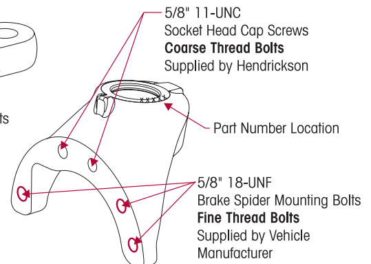
New Right Hand Upper Steering Knuckle
